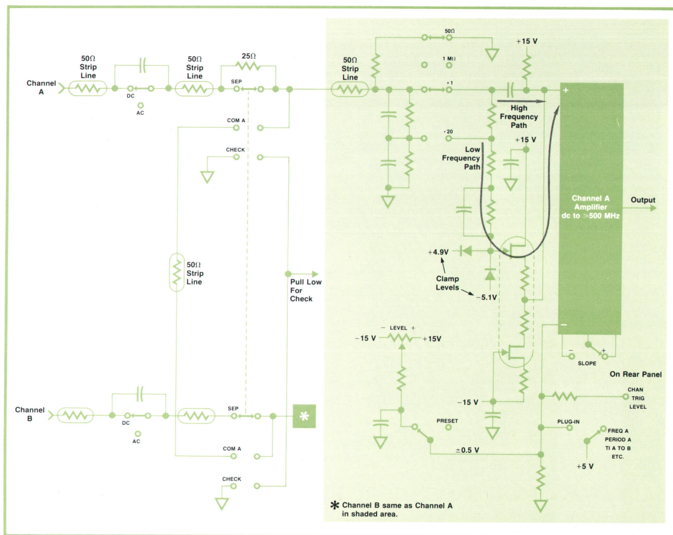
Fig. 7. Input amplifier and attenuator. Input impedance is switchable, 1\text{ M}\Omega/30\text{ pF} or 50\Omega .
